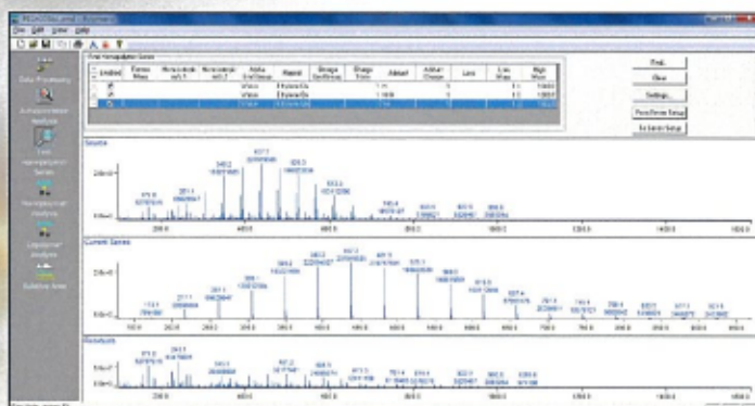
Find Homopolymer
