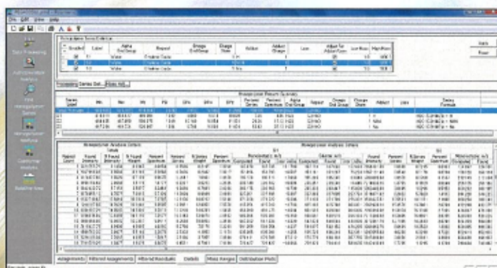
Homopolymer Details
